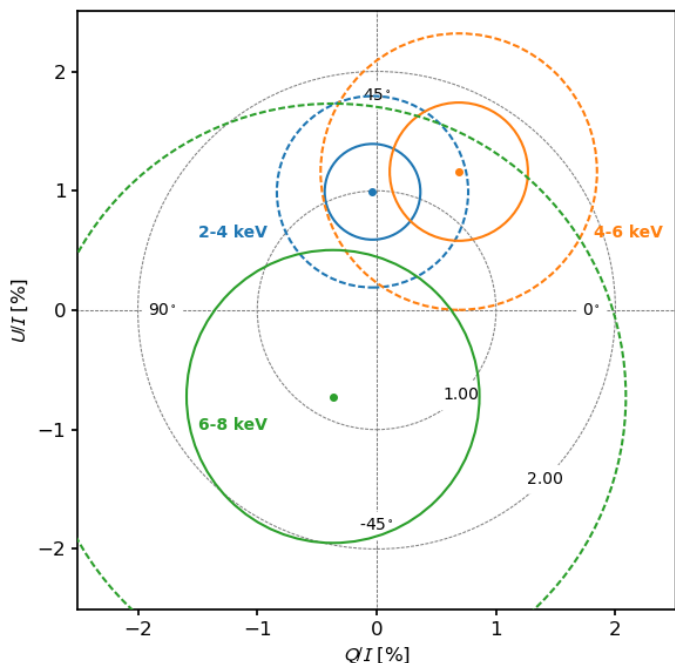
Fig. 3. Same details as in Fig. 2 for energy-dependent normalized Stokes parameters. Gray dotted circles represents loci of constant 1% and 2% PD. Blue, orange, and green circles represent the 2–4, 4–6 and 6–8 keV energy bands, respectively.
