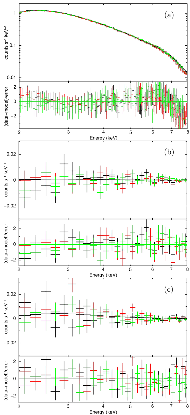
Fig. 4. EXO 2030+375 spectral energy distribution of the phase-averaged Stokes parameters I , Q , and U as observed by IXPE – panels (a), (b), and (c), respectively. Continuous lines in the top panels represent the best-fit model const×tbabs(powerlaw×polconst) reported in Table 1. Bottom panels show the residuals. Different colors represent different detectors – black for DU1, red for DU2, and green for DU3. Data have been rebinned and re-normalized for plotting purpose.
