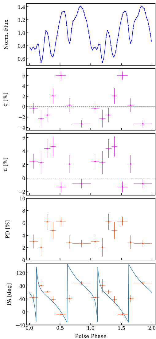
Fig. 6. Phase-resolved results of EXO 2030+375 in the 2–8 keV range, combining data from all IXPE DUs. From top to bottom, we show the pulse profile, normalized Stokes parameters q and u based on the polarimetric analysis, and the PD and PA, as obtained from the spectro-polarimetric analysis. The blue line in the PA panel corresponds to the best-fit rotating vector model (see Sect. 4.2).
