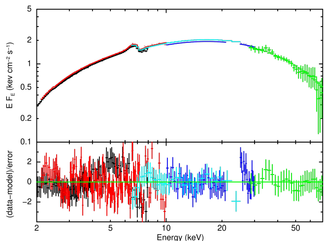
Fig. 5. Phase-averaged broadband spectrum of EXO 2030+375. Top: EXO 2030+375 unfolded EF_E spectrum as observed by IXPE , HXMT , and ART-XC . For plotting purpose, data from the three IXPE DUs are combined and re-normalized, and all spectra are rebinned. IXPE data are in red, HXMT LE, ME, and HE in black, blue and green, respectively, ART-XC data are in cyan. Bottom: Residuals of the best-fit model (also see Table 2).
