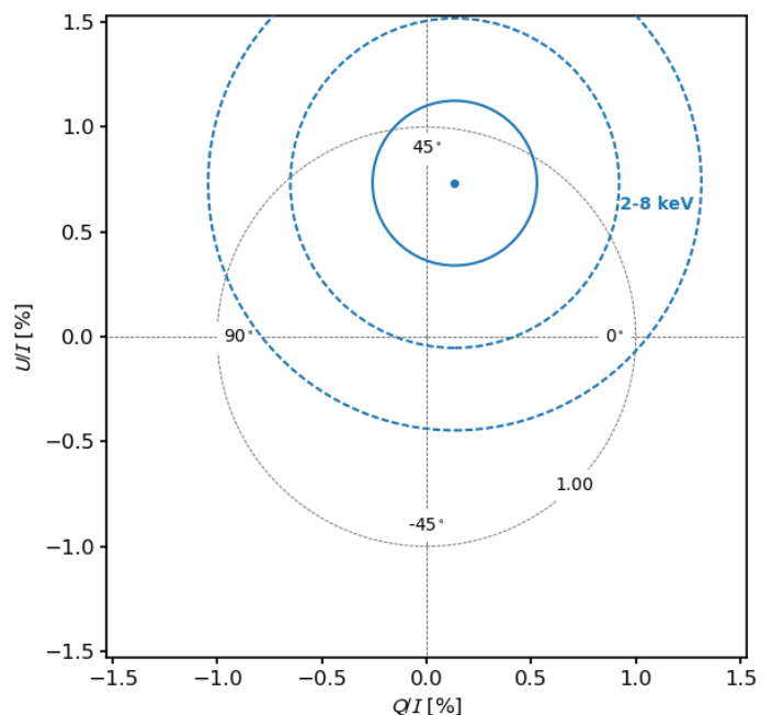
Fig. 2. Pulse phase-averaged normalized Stokes parameters U/I (y-axis) and Q/I (x-axis) over the 2–8 keV energy range. The 1\sigma , 2\sigma , and 3\sigma contours are plotted as concentric circles around the nominal value (continuous and dashed lines, respectively). The gray dotted circle represents loci of constant 1% PD, while radial lines are labeled for specific electric vector position angles (that is, the polarization angle, PA) with respect to north. The phase-averaged PD upper limit is about 2% at 99% c.l.
