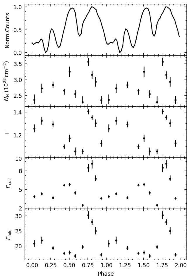
Fig. 7. Best-fit parameters for the broadband (2–50 keV) phase-resolved spectra of EXO 2030+375 as observed by HXMT . Panels from top to bottom show the pulse profile as observed by HXMT/LE in the 2–10 keV energy band; the column density, N_H ; the power-law photon index \Gamma ; the cutoff energy; and the folding energy (both in keV).
