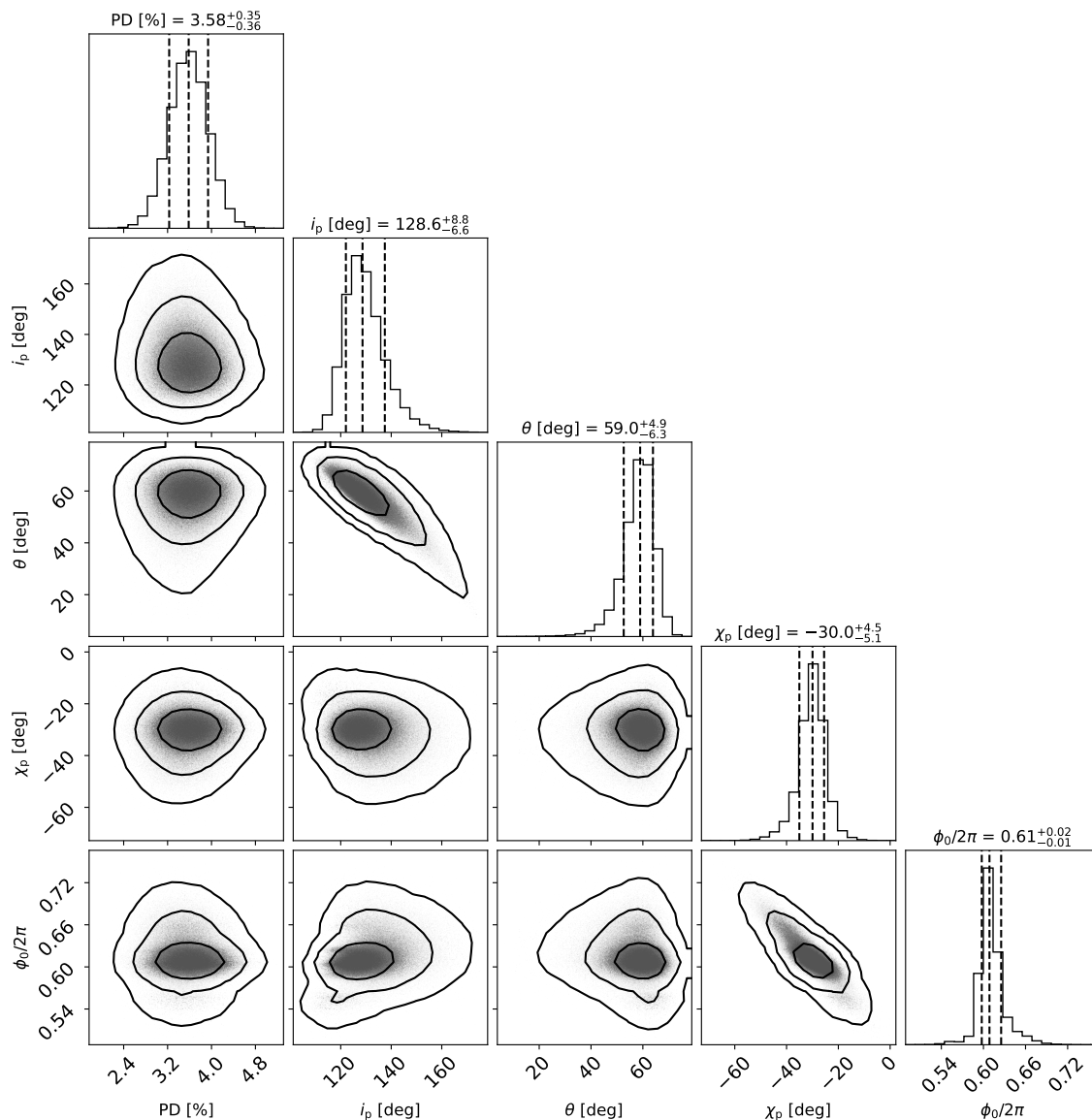
Fig. 8. Corner plot of the posterior distribution for the RVM parameters for the pulsar geometry obtained using the PA values. Parameters are the PD of radiation escaping from the magnetic pole, pulsar inclination, i_p ; magnetic obliquity, \theta ; position angle, \chi_p ; and the phase, \phi_0 . 2D contours correspond to 68%, 95% and 99% confidence levels. The histograms show the normalized 1D distribution for a given parameter derived from the posterior samples. The mean value and 1\sigma confidence levels for the derived parameters are reported above the corresponding histogram.
